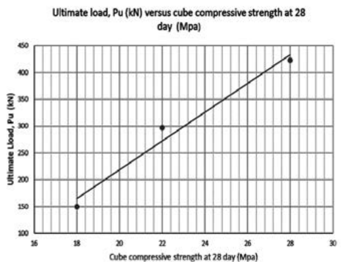
Figure 10: Ultimate load Carrying capacity versus cube compressive strength at 28 days
