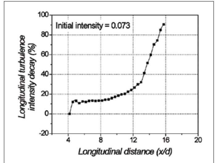
Figure 4: The longitudinal turbulence intensity decay along the centerline of the turbulent region.
